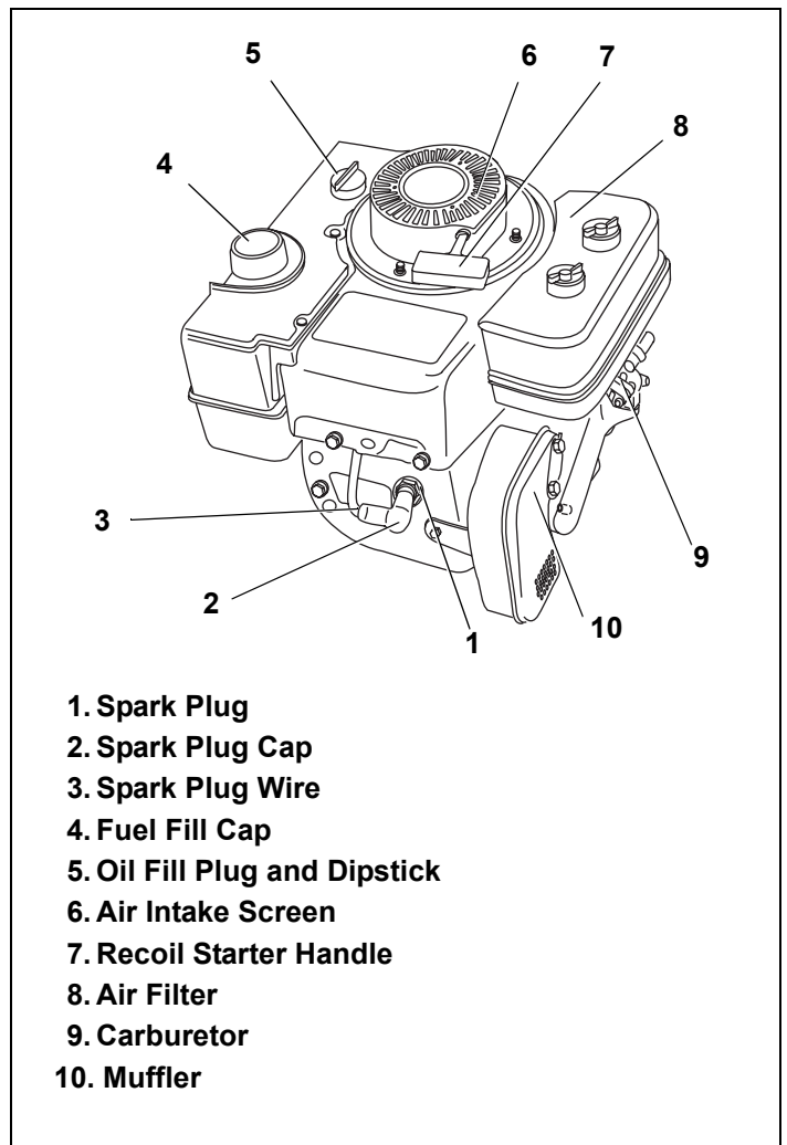
Figure 14. Engine Assembly with Oil Fill Dipstick
