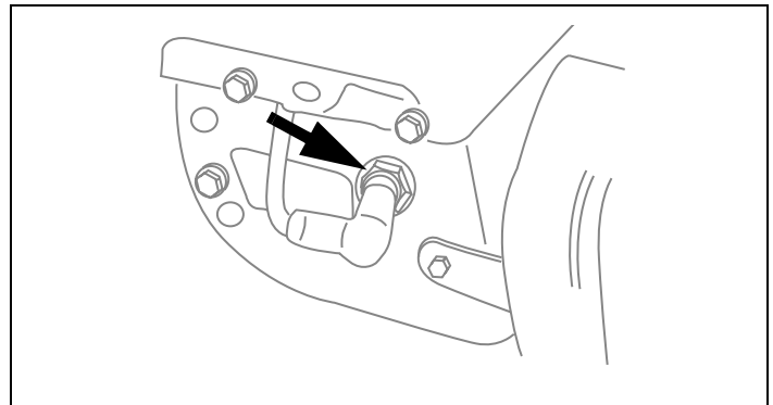
Figure 20. Typical Spark Plug Connection
